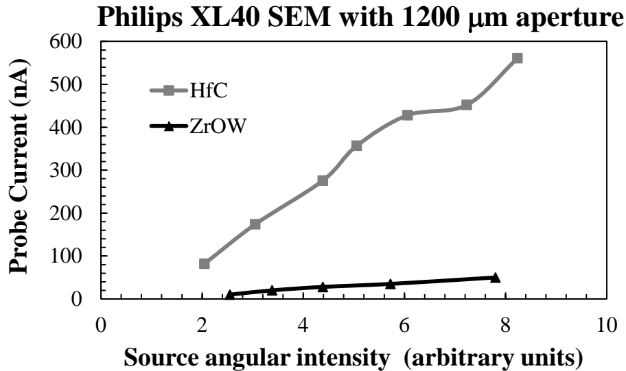
Figure 2: Beam current comparisons at several angular intensity levels.
