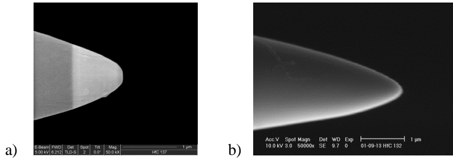
Figure 1: Micrographs of HfC(310) tips a) #137 and b) #132.
