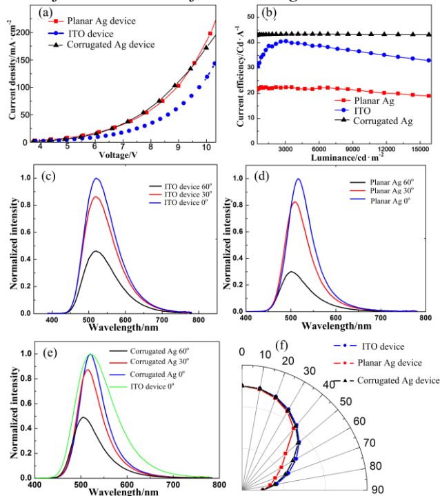
Figure 2: (a) Current density-voltage and (b) current efficiency- luminance characteristics for FOLEDs;The normalized electroluminescence spectra of (c) ITO device, (d)Planar Ag device and (e) corrugated Ag device;(f) emission patterns of devices.
