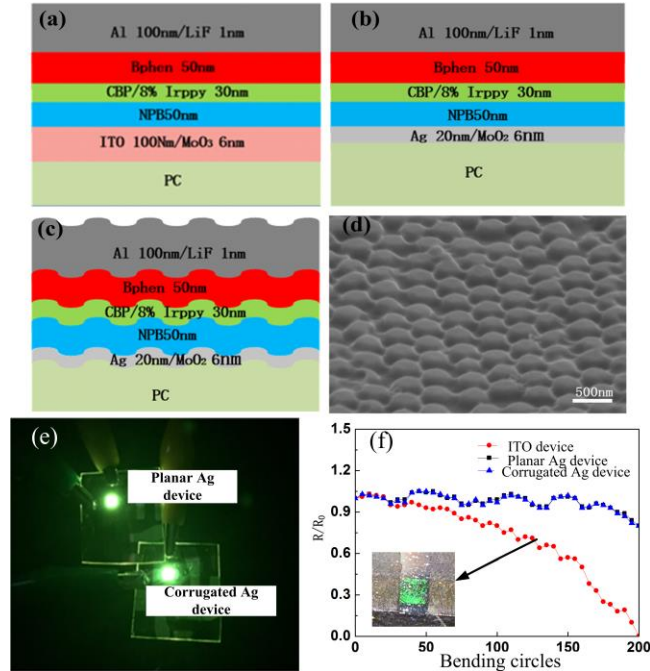
Figure 1. Structures for devices of (a) ITO anode (b) planar Ag anode and (c) corrugated Ag anode;(d) SEM image of corrugations on PC substrate through thermal NIL;(e) Working FOLEDs on planar and corrugated Ag substrates; (f) resistance properties for substrates after bending test.
